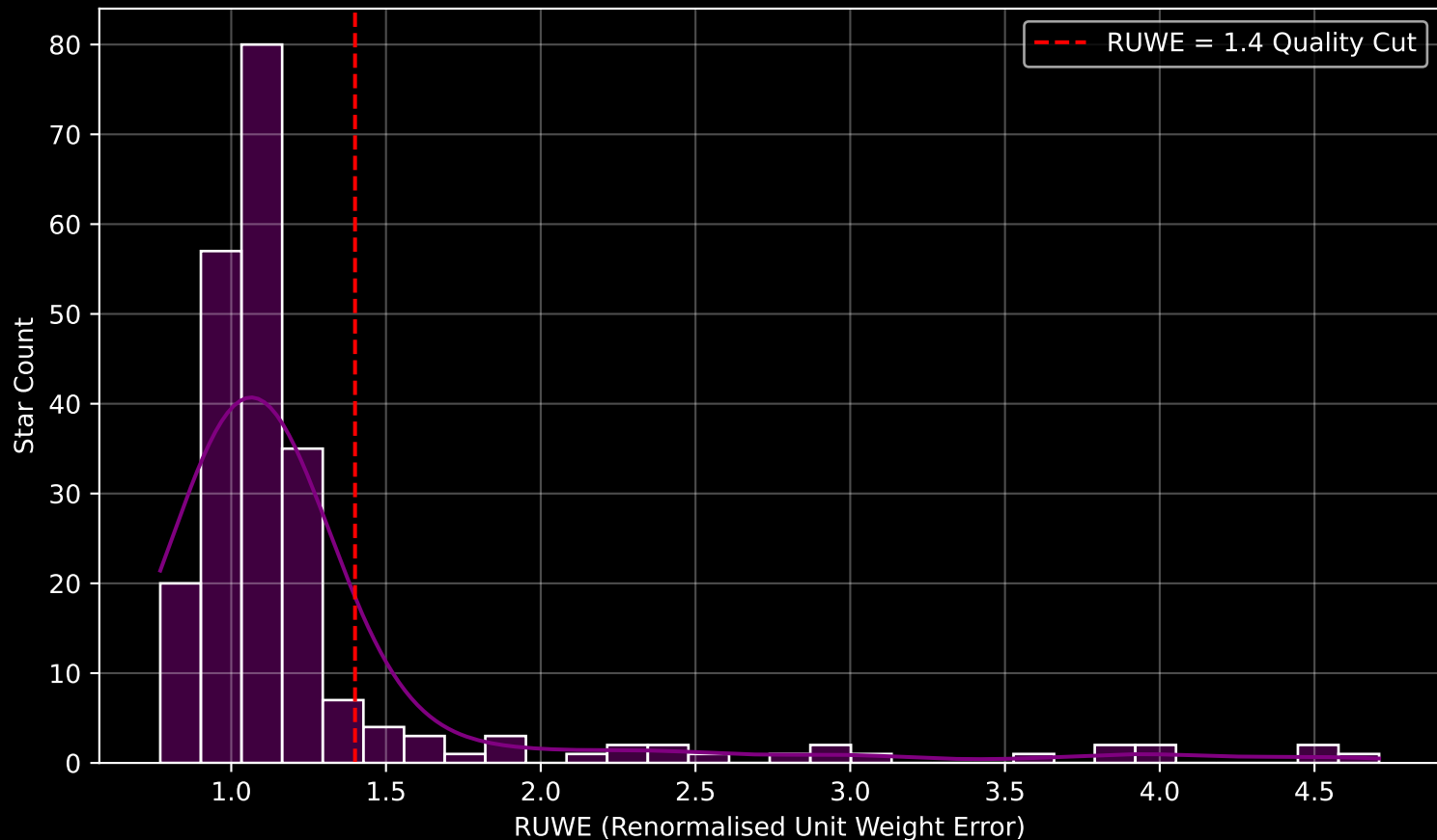
GALAH DR4 Field [7167] RUWE Distribution (n= 228)
