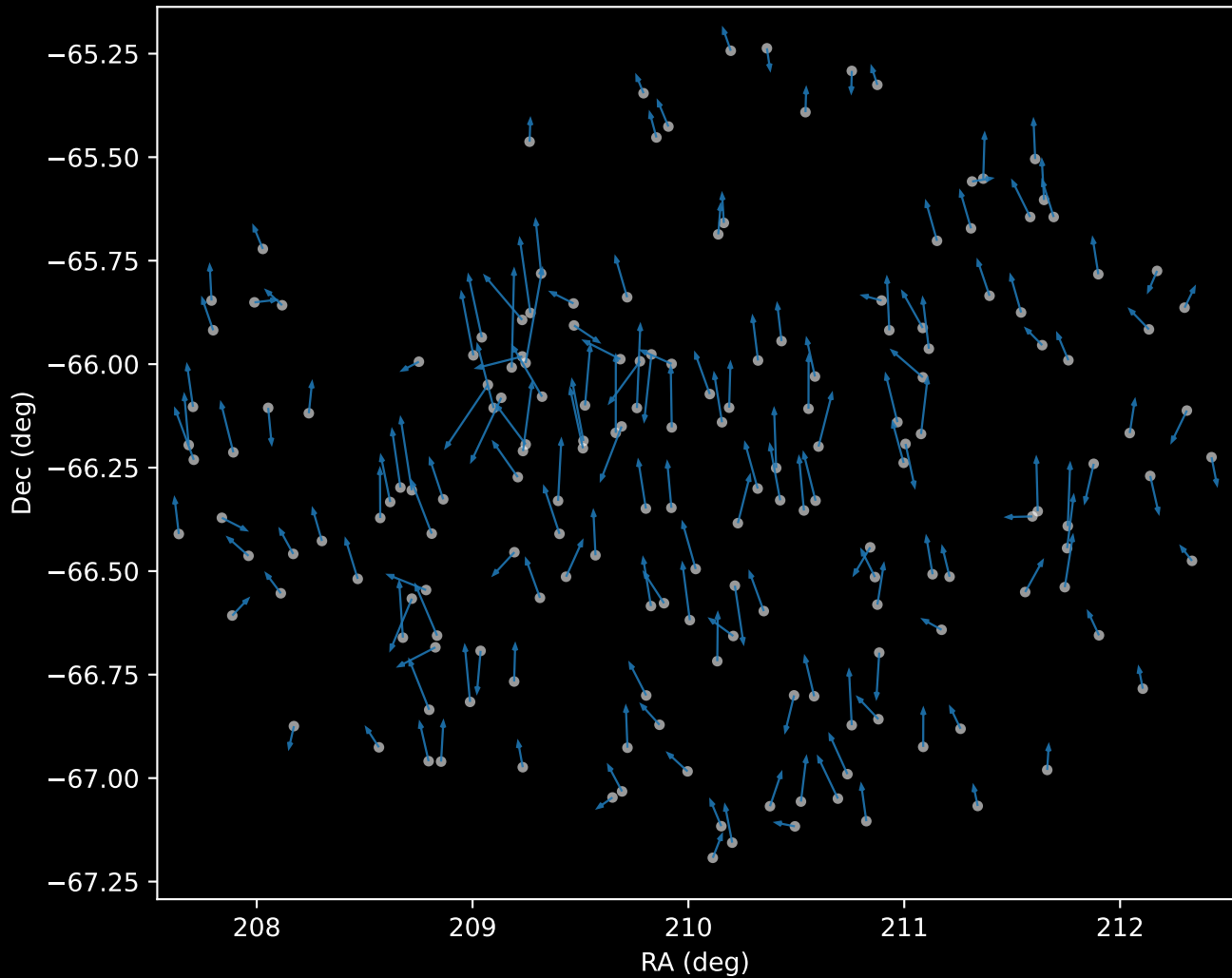
GALAH DR4 Cluster 0 Proper Motion Vectors (n=179)
