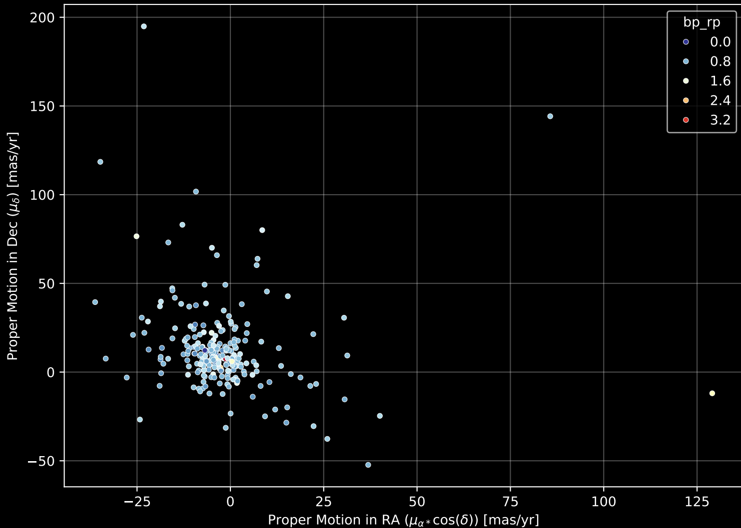
GALAH DR4 Field: [7167] Proper Motion Diagram (n= 239)
